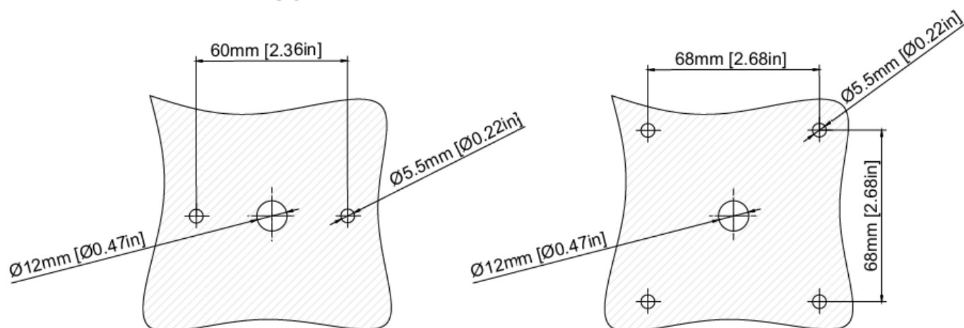
FRONTAL FIXING WITH 2 SCREW
