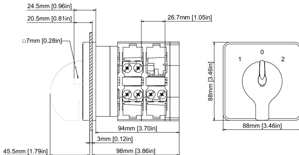
FRONTAL FIXING WITH 4 SCREW
